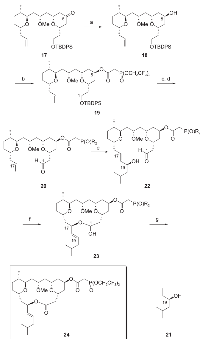
Scheme 5. Completion of the synthesis. a) L-Selectride, THF, -90^{\circ}\text{C} , 76%. b) (\text{CF}_3\text{CH}_2\text{O})_2\text{P}(\text{O})\text{CH}_2\text{CO}_2\text{H} , EDC, HOBt, \text{CH}_2\text{Cl}_2 , 92%. c) HCl, MeOH, 98%. d) Dess–Martin periodinane, \text{CH}_2\text{Cl}_2 , 95%. e) 21 , Hoveyda–Grubbs catalyst, 1,4-benzoquinone, \text{CH}_2\text{Cl}_2 , reflux, 70%. f) \text{Re}_2\text{O}_7 , \text{Et}_2\text{O} , 69%. g) PCC, \text{CH}_2\text{Cl}_2 , 81%. EDC = 1-(3-dimethylamino-propyl)-3-ethylcarbodiimide hydrochloride, HOBt = 1-hydroxybenzotriazole, PCC = pyridinium trioxochlorochromate, \text{R} = \text{OCH}_2\text{CF}_3 .
