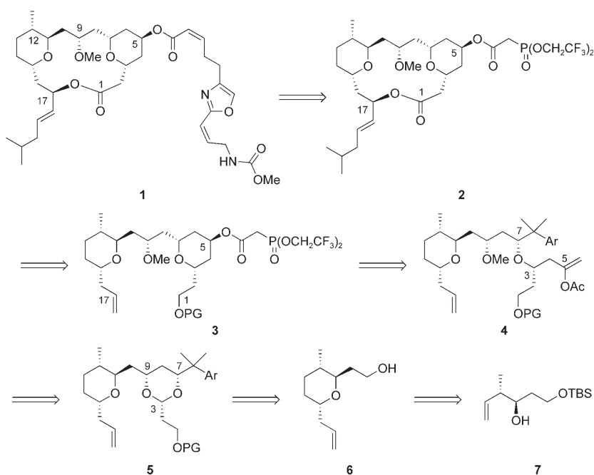
Scheme 1. Retrosynthetic analysis of leucascandrolide A ( 1 ). TBS = tert -butyldimethylsilyl, OAc = acetate, PG = protecting group, Ar = p -methoxyphenyl.
