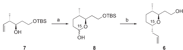
Scheme 2. Tetrahydropyran synthesis. a) \text{H}_2 , CO, [\text{Rh}(\text{CO})_2\text{acac}] , 6-diphenylphosphino-2-pyridone, THF, 1 atm, RT, 90% yield. b) Allyltrimethylsilane, \text{BiBr}_3 , \text{CH}_3\text{CN} , RT, 99% yield. TBS = tert -butyldimethylsilyl, acac = acetylacetonyl.
