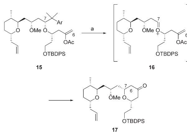
Scheme 4. ETIC reaction. a) Ceric ammonium nitrate, 4-Å M.S., \text{NaHCO}_3 , 1,2-dichloroethane, \text{CH}_3\text{CN} , 68%.
